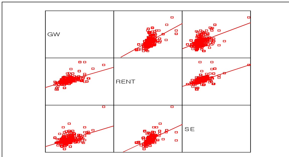
Figure 1: Scatter plot matrix of response variables and major explanatory variables
