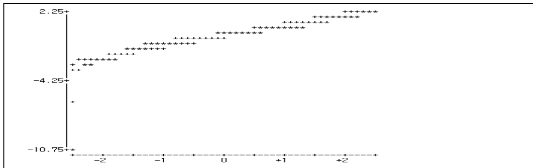
(b) Normal probability of Residue
