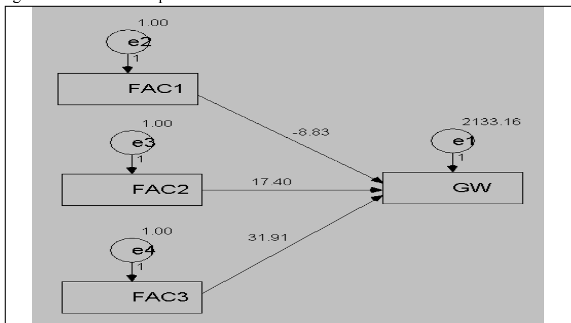
Figure 4: Structural Equations Model
