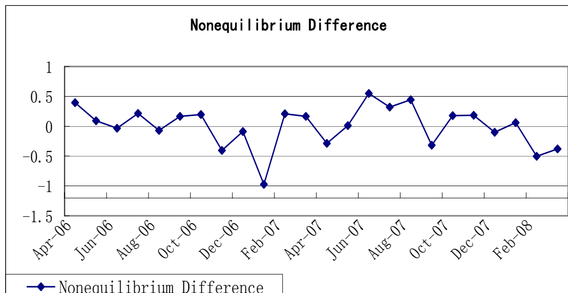
Figure 5: Nonequilibrium Difference Series
